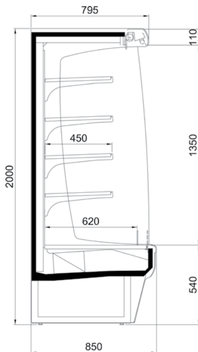
TWIST in Version H1
