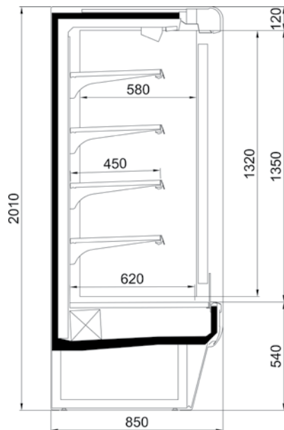
LG TWIST H1
